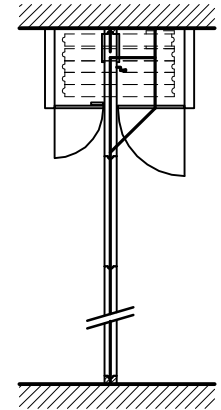
5. 'Z' system PANELS STACKED IN RECESS CUPBOARD
