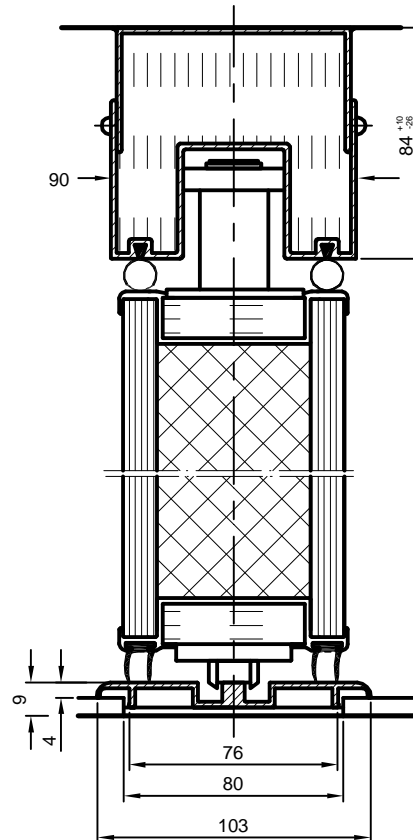
VERTICAL SECTION
