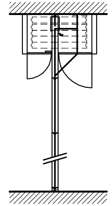
5. 'Z' system PANELS STACKED IN RECESS CUPBOARD
